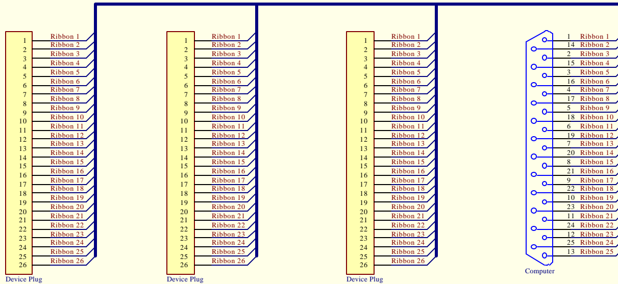
Sensor Ribbon Cables
