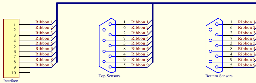
Sensor Ribbon Cables
